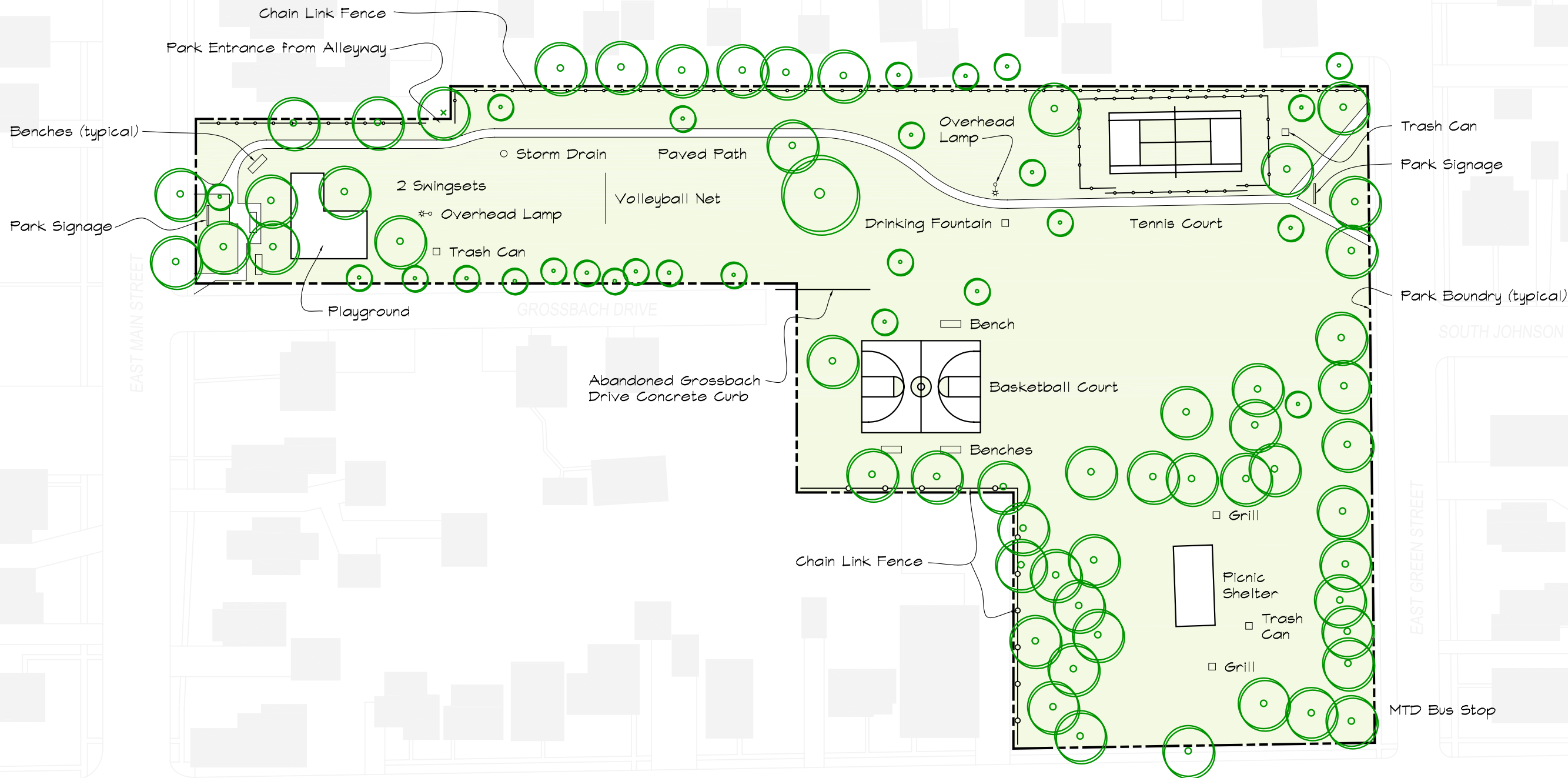
EXISTING PARK PLAN SCALE: 1" = 30'-0" 0 30 60 FEET
